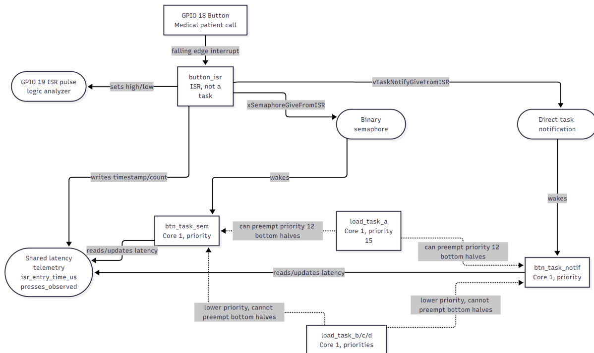
Fig. 1 System Diagram for Core 1
